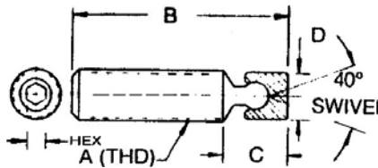
SWIVEL SCREW CLAMP WITH SMALL FOOT
